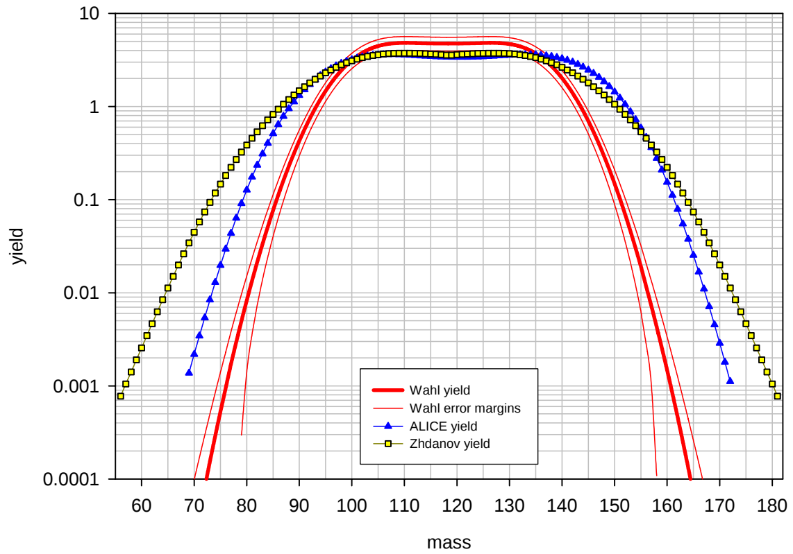
Benchmark B: ^{241}\text{Am} at 100 MeV, pre-neutron emission mass distribution
